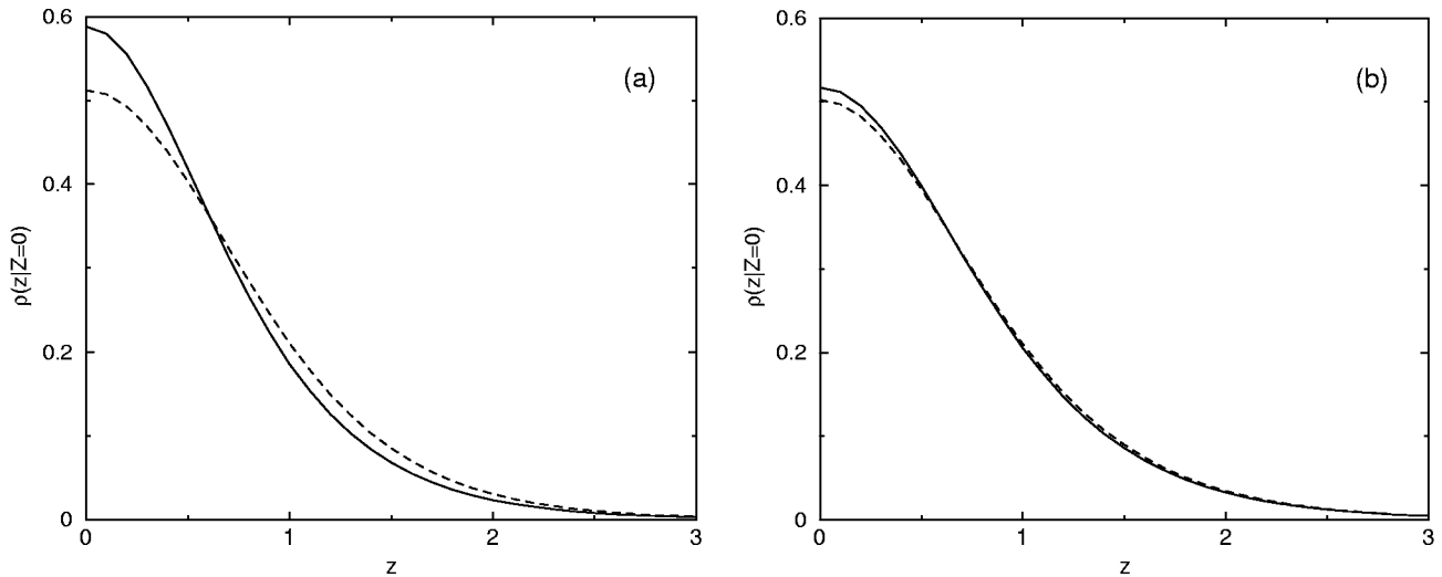
Figure 17: For the ground state of the one-dimensional attractive Bose gas, position dependence of the mean density of particles knowing that the center-of-mass of the gas is in Z = 0 . Solid line: exact result \rho(z|Z = 0) . Dashed line: mean-field approximation \rho^{\text{sb}}(z|Z = 0) . The position z is expressed in units of the ‘soliton’ radius l given in Eq.(512), and the linear density in units of N/l . The number of particles is (a) N = 10 and (b) N = 45 .
