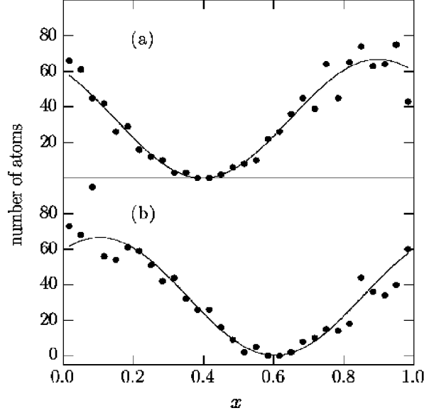
Figure 16: For two different Monte Carlo realizations (a) and (b) of the gedanken experiment, histogram of the measured positions of N = 1000 particles for an initial Fock state with N/2 particles in plane wave k_a and N/2 particles in plane wave k_b = -k_a [67]. The positions of the particles are expressed in units of 2\pi/(k_a - k_b) and are considered modulo 2\pi/(k_a - k_b) .
