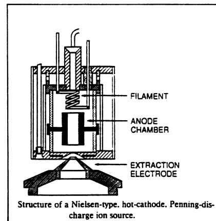
Figure VIII-1-5 - PIG axiale.
