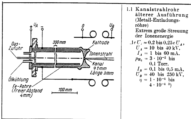
Figure VIII-1-1 - Source capillaire.
