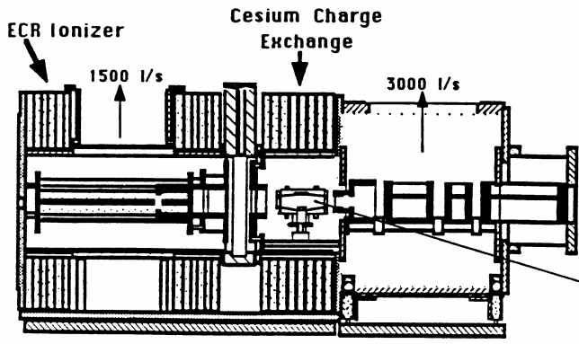
Figure 1.1.11a - Arrangement of a CE Cs cell.
