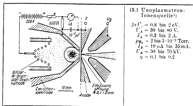
Figure VIII-1-2 - Unoplasmatron
