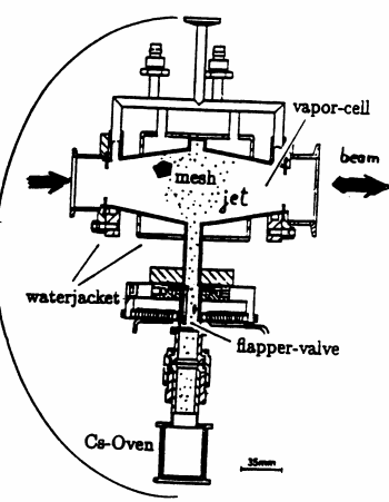
Figure 1.1.11b - Cesium cell.
