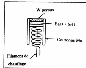
Figure II-1-19 - Cathode L.
