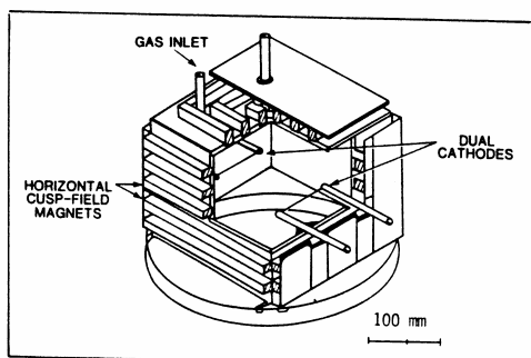
Figure VIII-1-16 - Source "multicusp".
