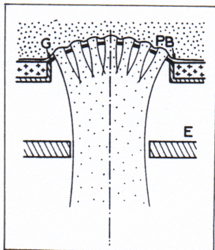
Figure XII-5-5 - Extraction multiouverture.
