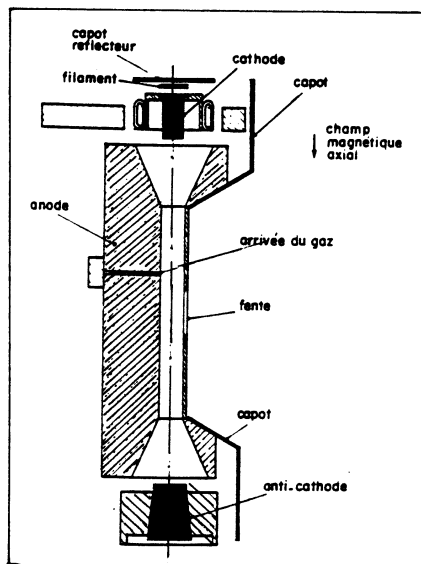
Figure VIII-1-4 - PIG radiale.
