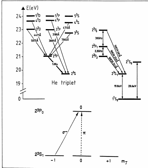
Figure 2.2.2 - Scheme of the radiation polarizations for the 2^3S_1 \rightarrow 2^3P_0 transition.
