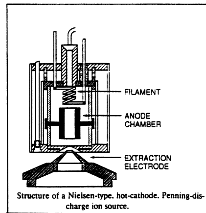
Figure VIII-1-5 - PIG axiale.
