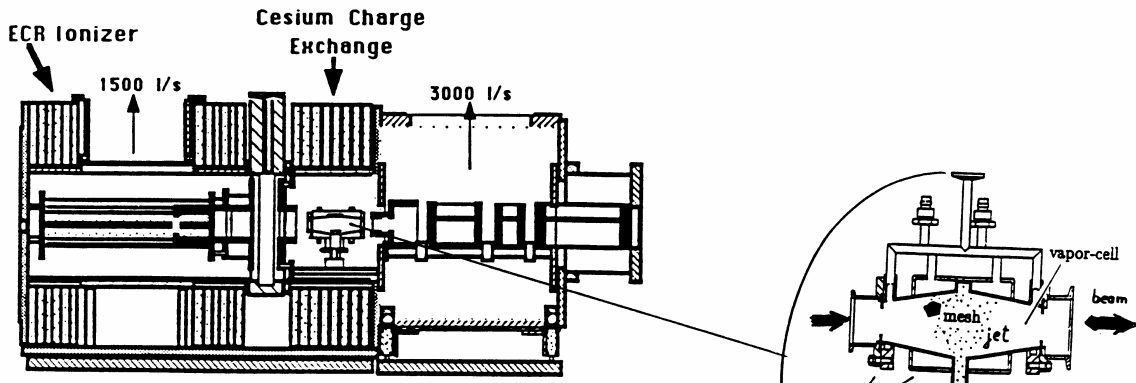
Figure 1.1.11a - Arrangement of a CE Cs cell.
