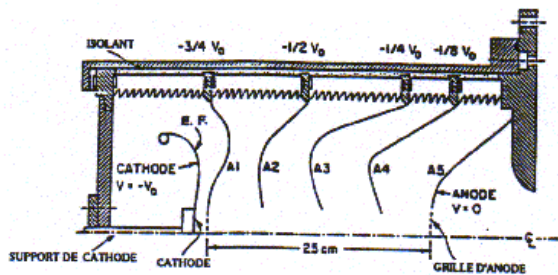
Figure III-2-6 - Canon diode.
