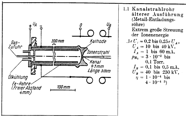
Figure VIII-1-1 - Source capillaire.
