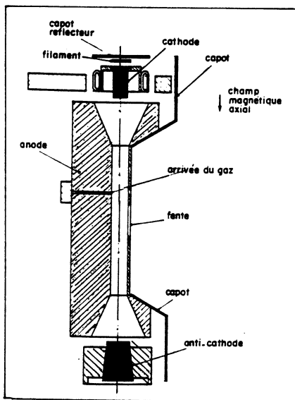
Figure VIII-1-4 - PIG radiale.
