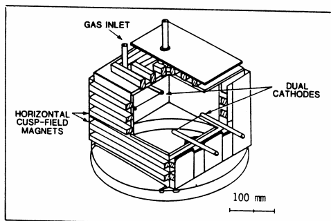
Figure VIII-1-16 - Source "multicusp".
