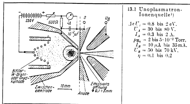
Figure VIII-1-2 - Unoplasmatron
