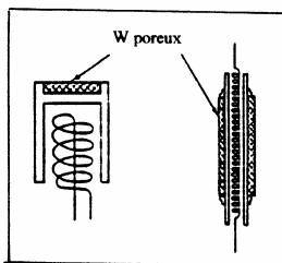
Figure II-1-21 - Cathodes A, B et M.
