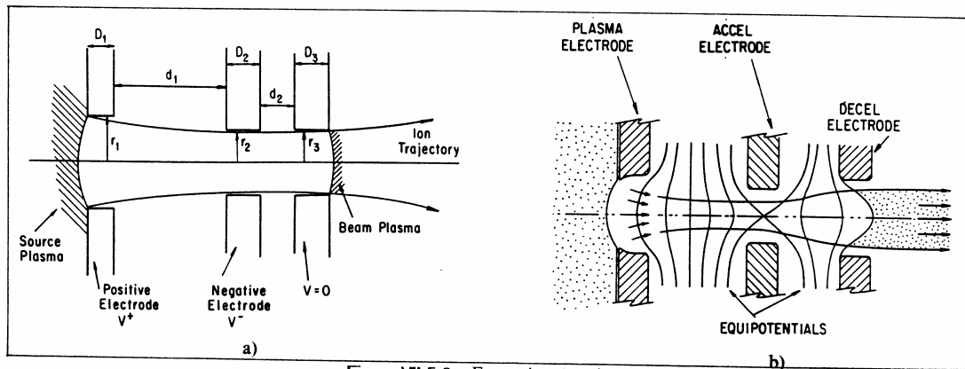
Figure XII-5-8 - Extraction Accel-Decel.
