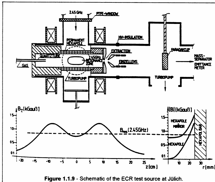
Figure 1.1.9 - Schematic of the ECR test source at Jülich.
