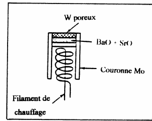
Figure II-1-19 - Cathode L.
