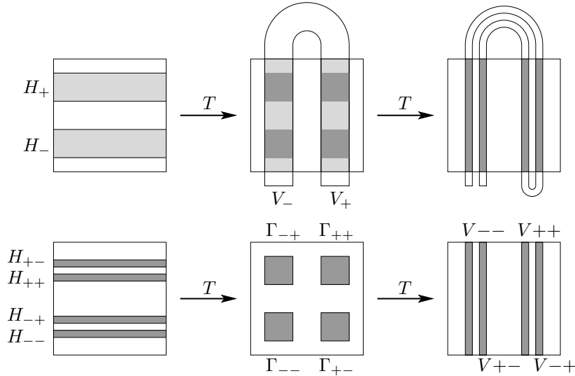
FIGURE 4.5. The horseshoe map T maps the rectangles H_\pm of the unit square Q to the rectangles V_\pm . If \Gamma_{\varepsilon_0\varepsilon_1} = V_{\varepsilon_0} \cap H_{\varepsilon_1} , one also has T(H_{\varepsilon_0\varepsilon_1}) = \Gamma_{\varepsilon_0\varepsilon_1} and T(\Gamma_{\varepsilon_0\varepsilon_1}) = V_{\varepsilon_0\varepsilon_1} .
