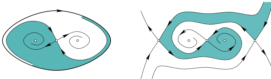
FIGURE 2.6. Examples of basins of attraction.
