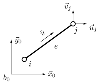
Figure A.8 - Bases e et b_0
