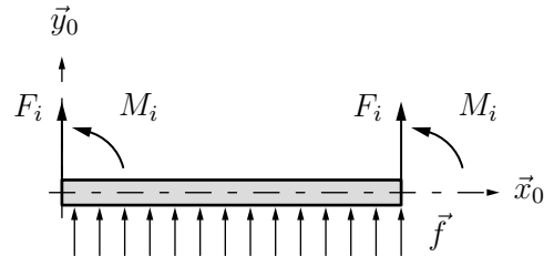
Figure 3.6 - Efforts extérieurs
