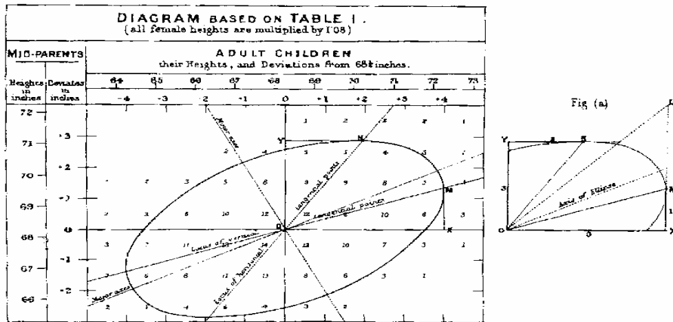
Figure 8.7. Galton's smoothed version of Table 8.1, with one of the "concentric and similar ellipses" drawn in. The geometric relationship of the two regression lines to the ellipse is also shown. (From Galton, 1886a.)
