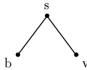
FIGURE 2. Dynkin diagram A_3 as fusion graph
