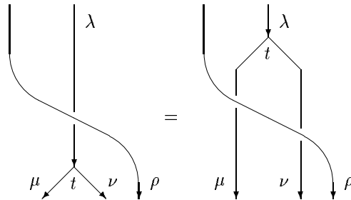
FIGURE 10. The second braiding fusion equation for over-crossings
