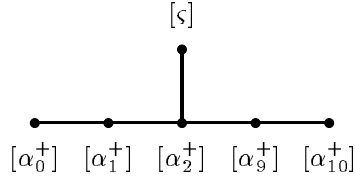
FIGURE 14. SU(2)_{10} \subset SO(5)_1 : Fusion graph of [\alpha_1^+] on the chiral system E_6^+
