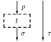
FIGURE 4. An intertwiner t \in \text{Hom}(\rho, \sigma) \subset \text{Hom}(\rho\tau, \sigma\tau)
