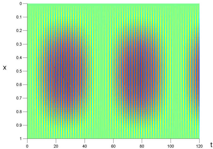
Figure 3.5: Time evolution of solution (3.52) for h = 1/61 ( N = 60 ) and 0 \leq t \leq 120 . It is clear that, according to the figure, the solution seems to exhibit a time-periodicity property with period \tau of the order of \tau \sim 50 . Note however that all solutions of the wave equation are time-periodic of period 2. In the figure it is also clear that fronts propagate in space at velocity of the order of 1/50 . This is in agreement with the prediction of the theory in the sense that high frequency wave packets travel at a group velocity of the order of h .
