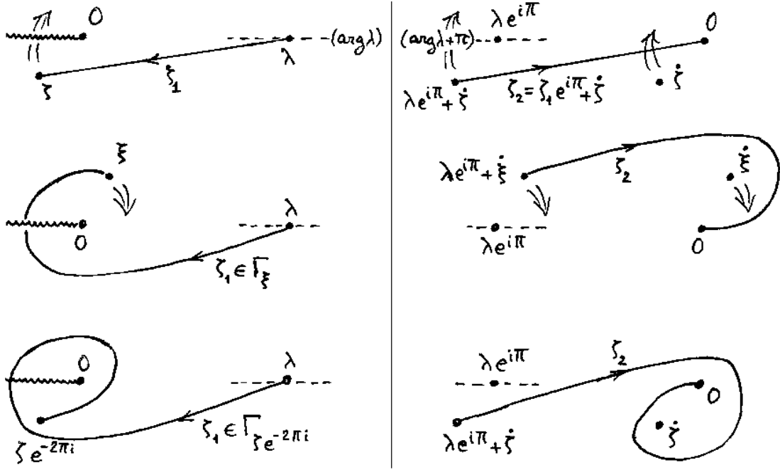
Figure 13: Analytic continuation of \check{\varphi}_{3,\lambda} . (Left: three examples of path \Gamma . Right: the corresponding paths followed by \zeta_2 = \zeta_1 e^{i\pi} + \check{\zeta} ).
