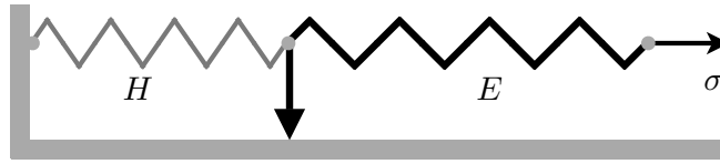
FIGURE 3.6 – L'assemblage ressort–patin–ressort.
