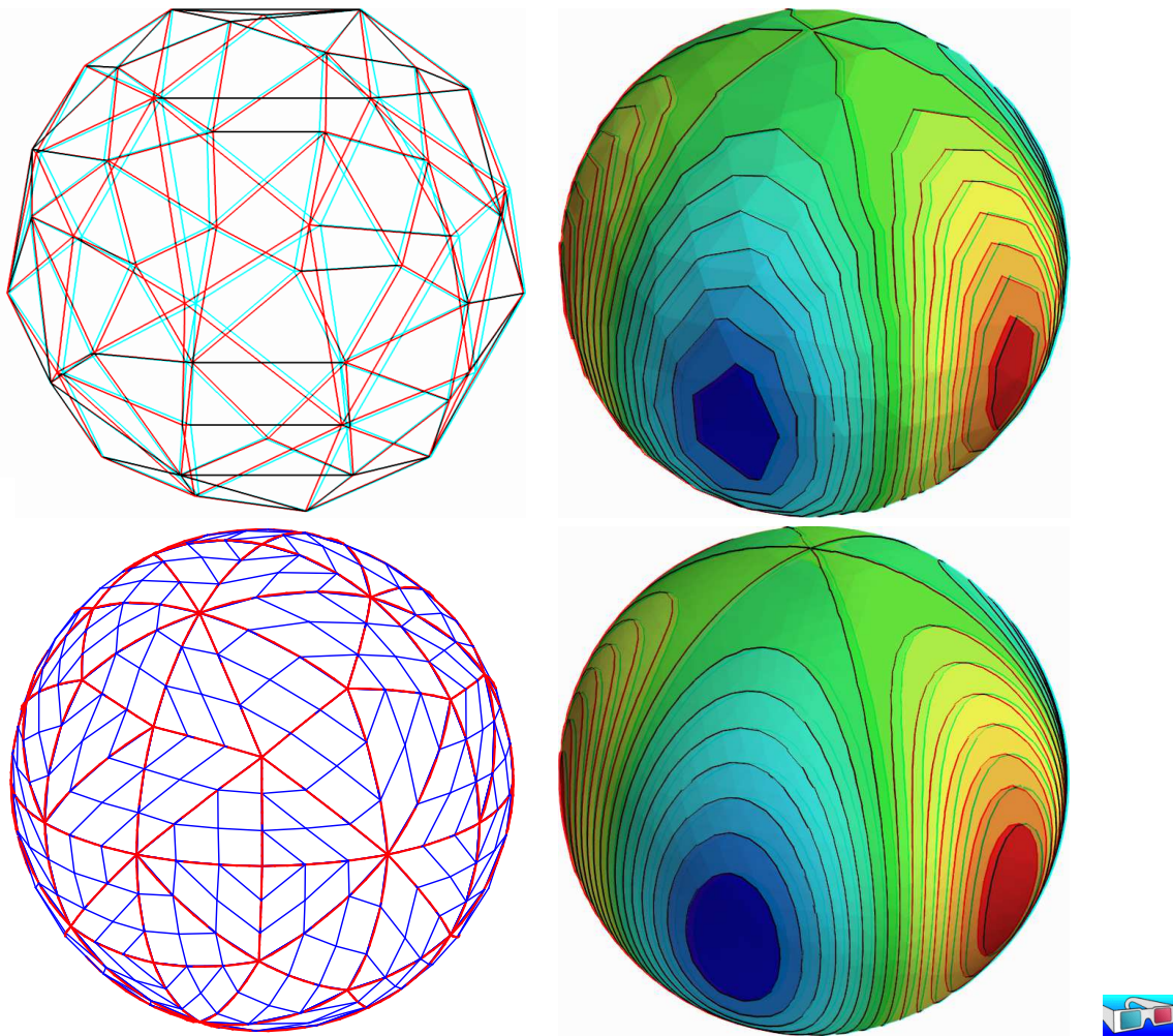
Figure 7.1: Helmholtz-Beltrami problem: high-order curved surface mesh and its corresponding isoparametric solution: (top) order = 1 ; (bottom) order = 3 .
