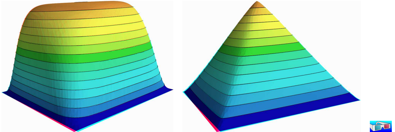
Figure 8.7: The p -Laplacian for d = 2 : elevation view for p = 1.15 (left) and p = 7 (right).
