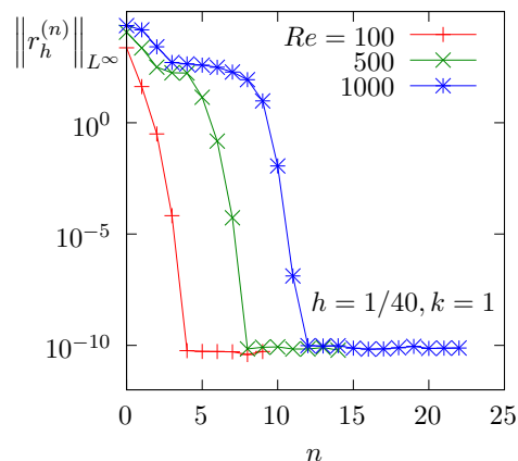
Figure 4.15: The discontinuous Galerkin method for the Navier-Stokes problem on the driven cavity benchmark when k = 1 and d = 2 : convergence of the damped Newton algorithm.
