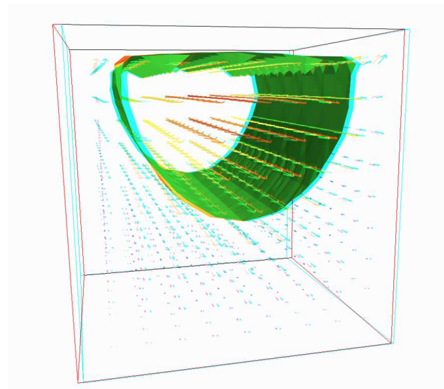
Figure 2.8: The stream function visualization: isolines for d = 2 , and combined vectors and isonorm surface for d = 3 .
