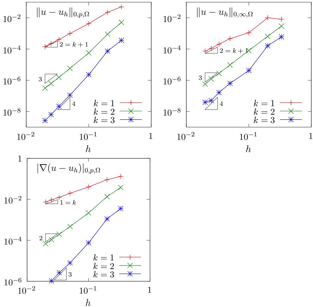
Figure 3.15: The p -Laplacian for d = 2 : error analysis.
