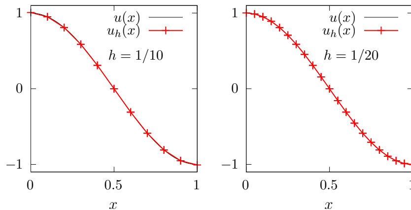
Figure 4.10: The discontinuous Galerkin method for the Poisson problem when k = 1 and d = 1 .
