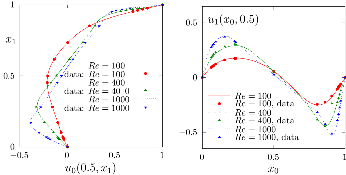
Figure 2.21: Navier-Stokes: velocity profiles along lines passing through the center of the cavity, compared with data from Ghia et al. [1982]: (a) u_0 along the vertical line; (b) u_1 along the horizontal line.
