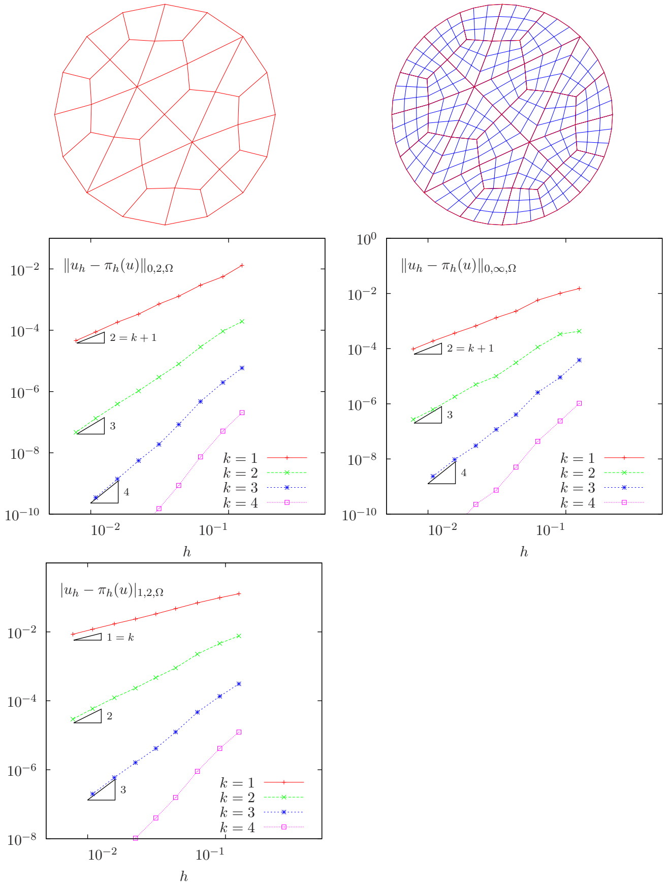
Figure 9.3: Curved domains (quadrangles): error analysis in L^2 , L^\infty and H^1 norms.
