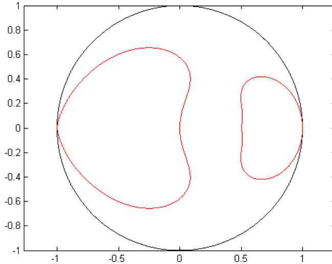
FIGURE 4. The eigenvalues of M(q(\eta)) in red and the unit circle in black.
