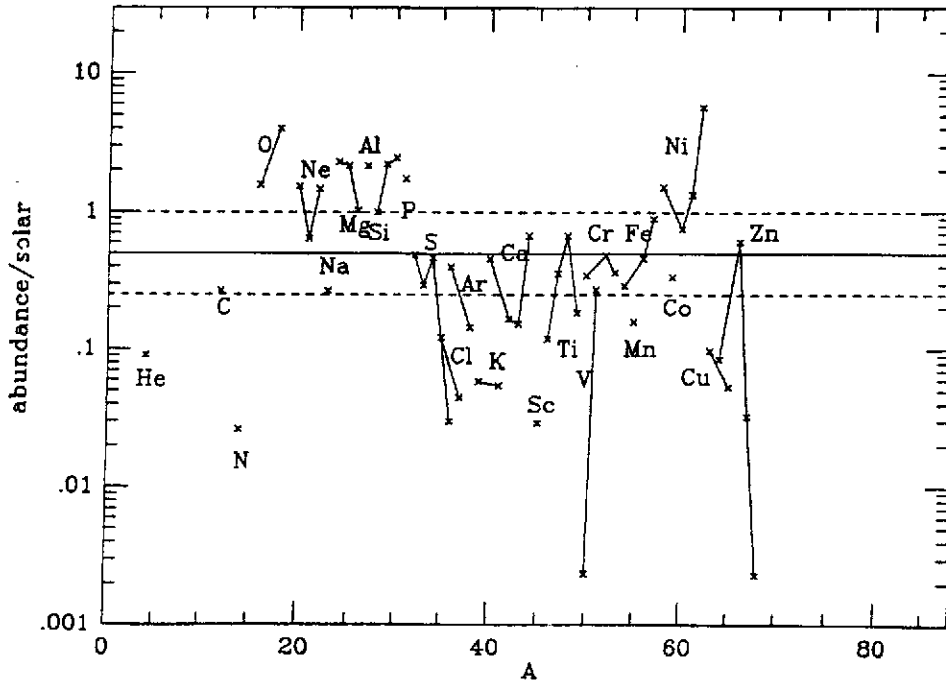
Fig.30. Calculated abundances of the Z \leq 30 in the ejecta of the (Type II) supernova SN1987A (see Sect. 7) compared to the bulk SC, and normalized to the solar ^{28}\text{Si} abundance (from Thielemann et al. 1989). Different isotopes of the same element are connected by lines.
