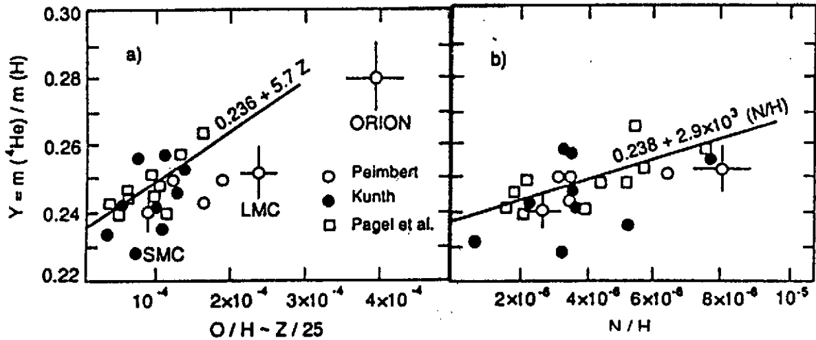
Fig.9. Observations of the {}^4\text{He} abundance in HII regions, as a function of the abundances of O [part a)] and N [part b)]. Extrapolation to zero abundances for O or N allows then to estimate the primordial {}^4\text{He} mass fraction: 0.23 < Y_p < 0.24 .
