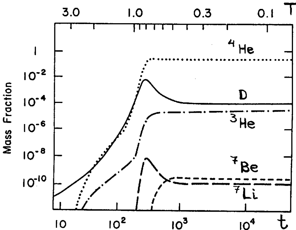
Fig.7. Evolution of the abundances of light nuclides in standard Big Bang nucleosynthesis calculations, as a function of time t (down, in s), or temperature T (up, in 10^9 K). Nucleosynthesis really starts at t \sim 200 s, with the breaking of the "deuterium bottleneck" (see text). {}^7\text{Be} eventually decays to {}^7\text{Li} , with a half-life of \sim 54 days.
