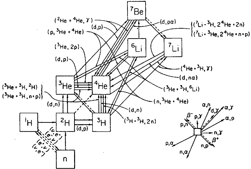
Fig.6. Reaction network with the most important reactions for standard primordial nucleosynthesis models. Unstable nuclei with mass A = 8 do not allow to go beyond {}^7\text{Li} in such models.
