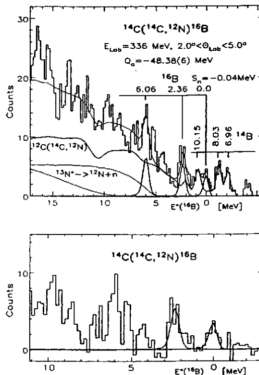
Figure 2: Top panel: Excitation energy spectrum for the reaction ^{14}\text{C}(^{14}\text{C},^{12}\text{N})^{16}\text{B} [56]. Note the background arising from reactions on the small amount of ^{12}\text{C} present in the target. Bottom panel: Same spectrum after subtraction of a spectrum taken using a ^{12}\text{C} target.
