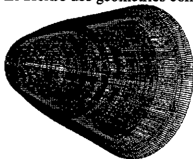
CMS
