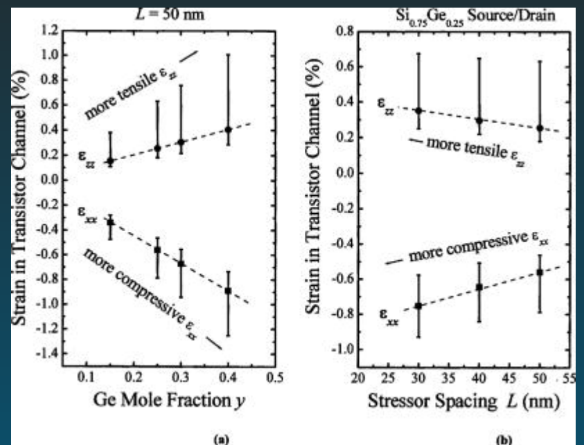
Evolution of channel strain as a function of the Ge fraction and the spacer with
