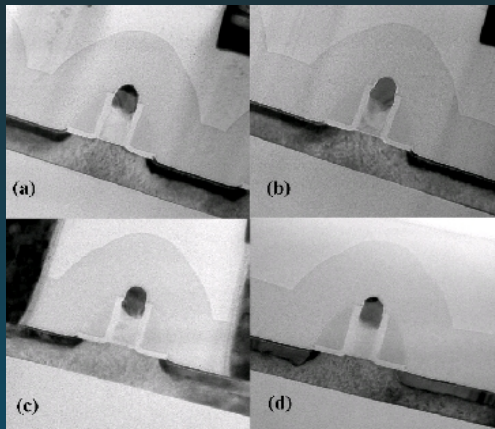
Figure 1. TEMs of 35nm gates with highly stressed ESL films as a function of gate poly pitch: (a) 0.26 \mu\text{m} , (b) 0.38 \mu\text{m} , (c) 0.63 \mu\text{m} , (d) 1.04 \mu\text{m} .
