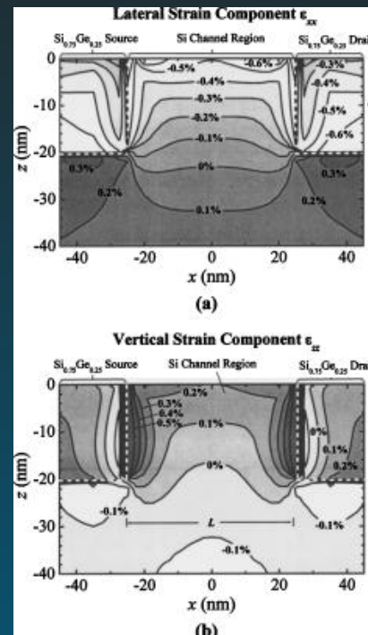
Lateral & Vertical strain induced
