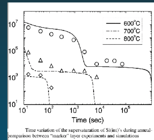
Evolution of Si interstitials as a function of the time
