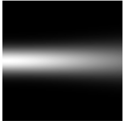
Paraxial Beam
