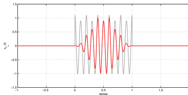
FIGURE 2.35 – Signal w_{hanning}(t)x_{T_a}
