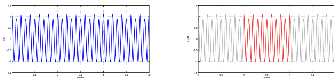
FIGURE 2.28 – Signal x (gauche) et signal x_{T_a} (droite)
