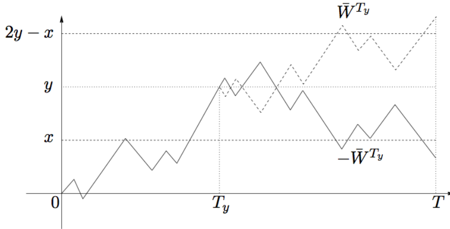
Figure 1.3: Brownian motion ( W_{T_y+t} = \bar{W}_t^{T_y} + y : t \in \mathbb{R}^+ ) starting from y and its symmetric path.
