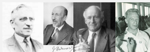
Lebesgue Hadamard Schwartz Sobolev
