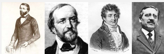
Riemann Dirichlet Fourier Lebesgue
