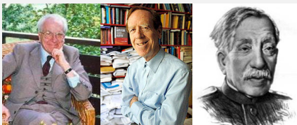
Argyris Strang Galerkin
