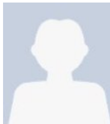
Paris
