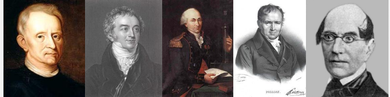
Hooke
