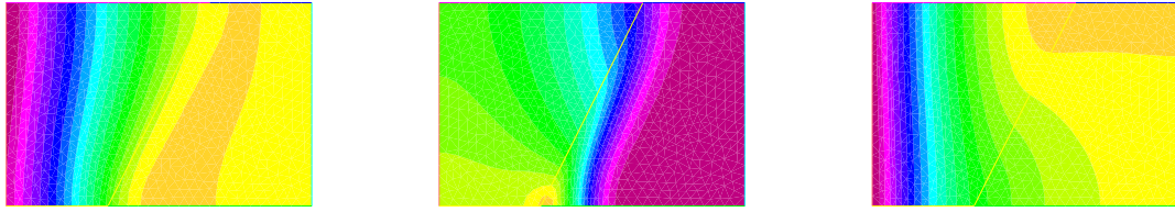
\Re(p)
