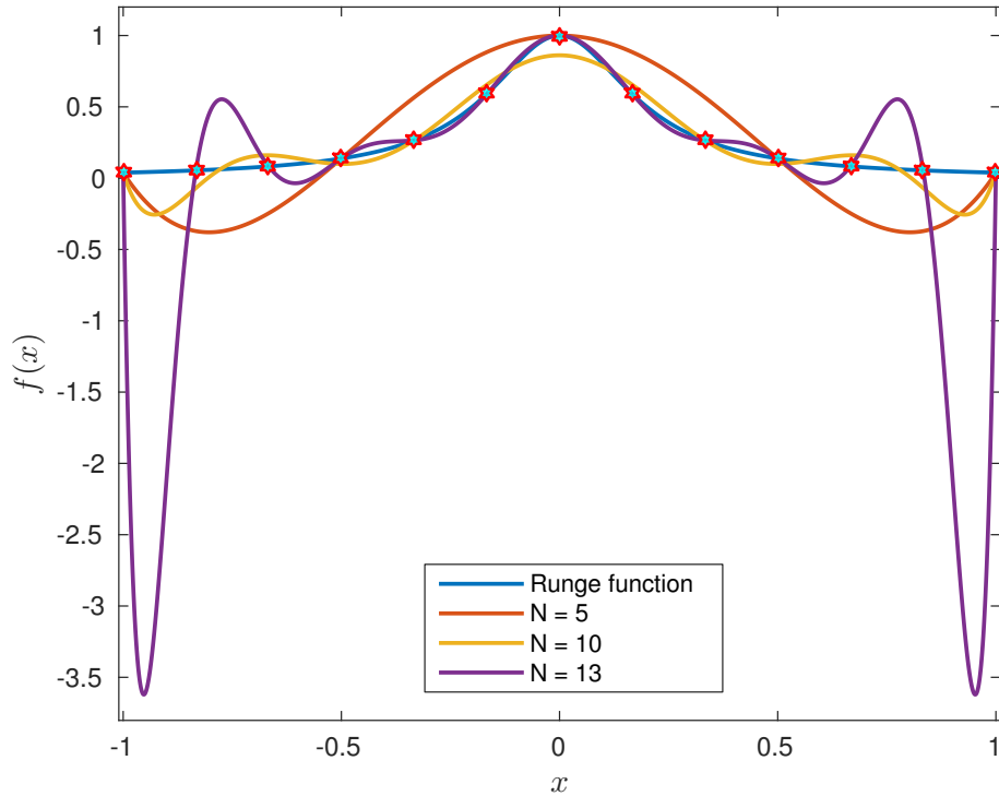
Figure 2. Interpolation of the RUNGE function f(x) = \frac{1}{1+25x^2} on a sequence of successively refined of uniform grids. One can observe the divergence phenomenon close to the interval boundaries x = \pm 1 .
