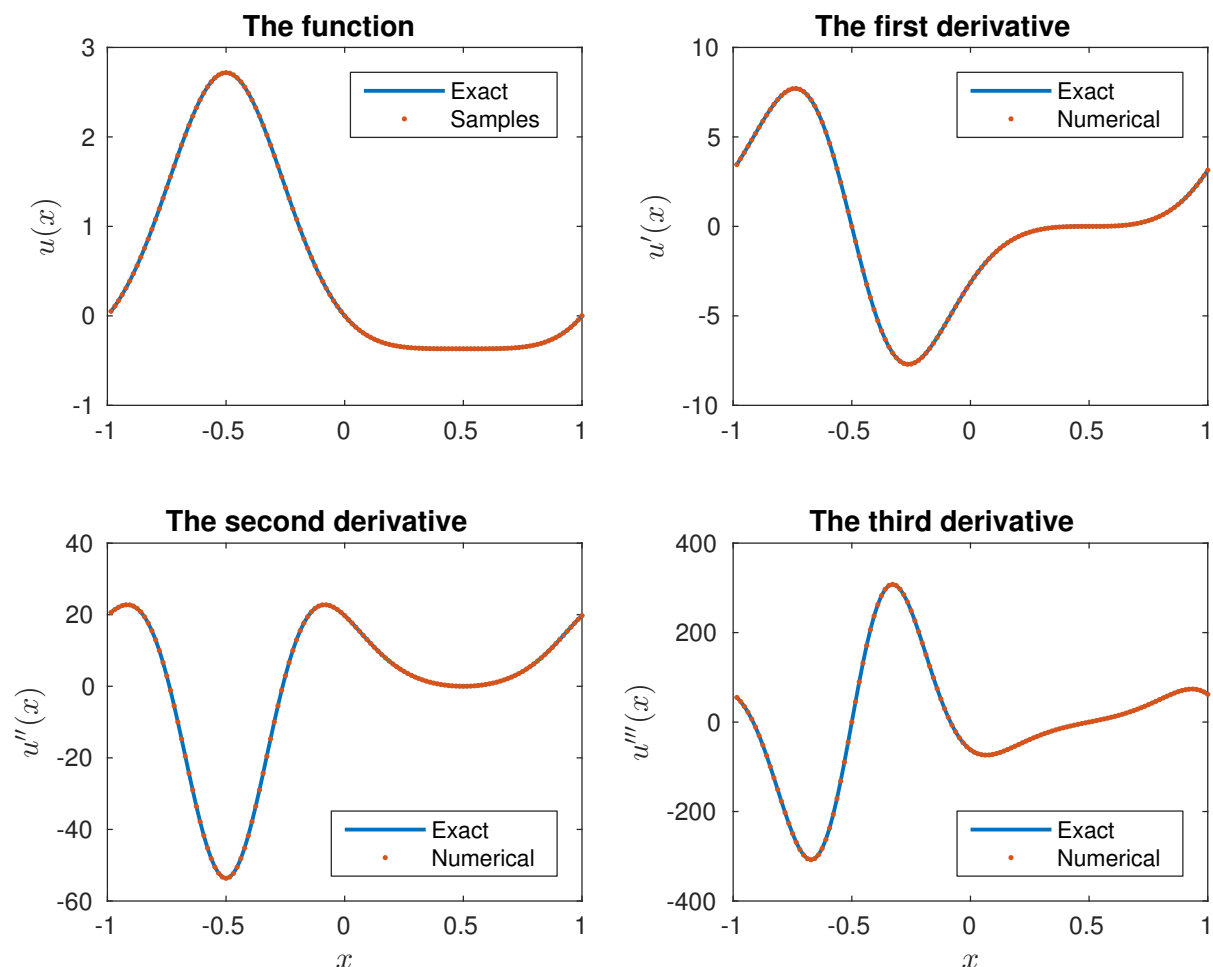
Figure 7. Numerical differentiation of a periodic function (4.9) using the FOURIER collocation spectral method. We use 128 collocation points. The agreement is perfect up to graphic accuracy.
