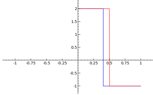
Figure 3: Solution à T = 1 , h = 0.01
