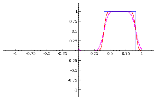
Figure 1: Solutions à t = 0.4 , h = 0.05
