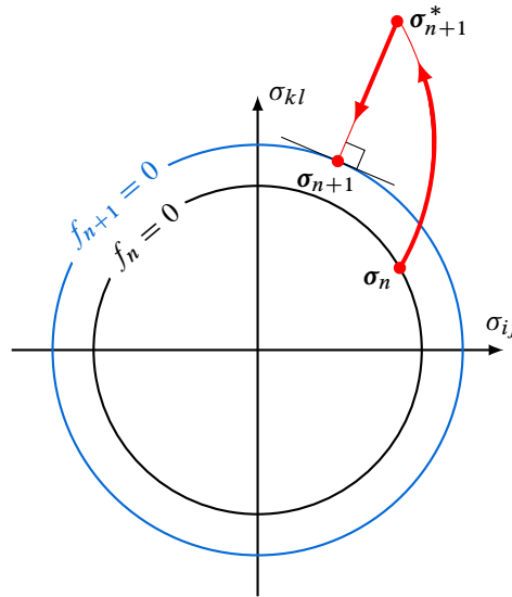
Figure 4.4 – Retour radial
