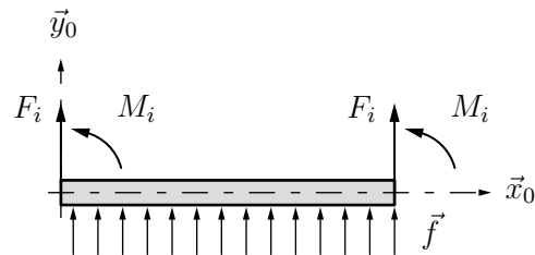
Figure 3.6 - Efforts extérieurs
