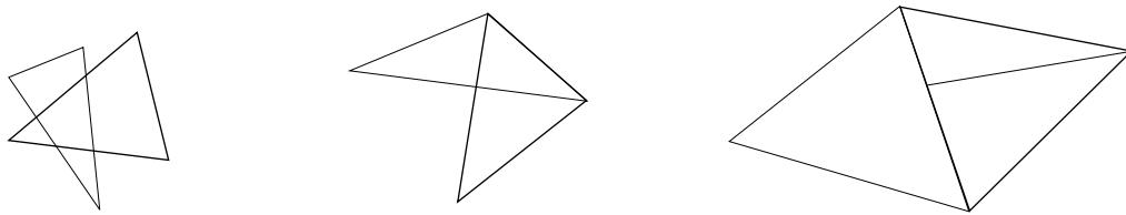
FIGURE 12.5: Maillage non conforme : situations interdites
