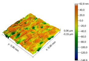
Figure: Surface obtained by polishing ( z \times 500 ), WLI, L = 0.9\text{mm} , \Delta x = 0.9\mu\text{m} .
