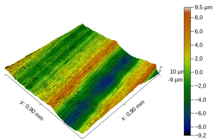
Figure: Surface obtained by rough milling ( z \times 5 ), WLI, L = 0.9\text{mm} , \Delta x = 0.9\mu m .
