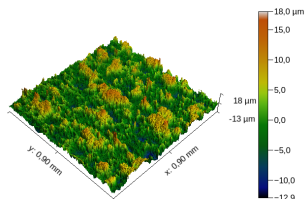
Figure: Surface obtained by electroerosion ( z \times 5 ), WLI, L = 0.9\text{mm} , \Delta x = 0.9\mu m .
