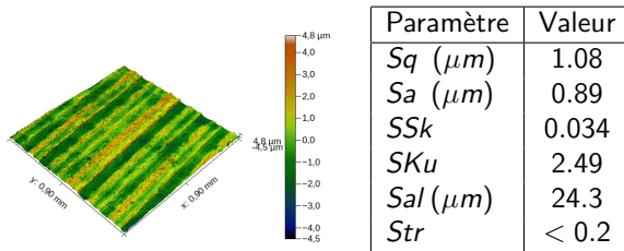
Figure: Surface obtained by fine milling ( z \times 5 ), WLI, L = 0.9\text{mm} , \Delta x = 0.9\mu\text{m} .
