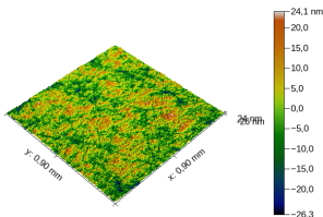
Figure: Surface obtained by mirror polishing ( z \times 500 ), WLI, L = 0.9\text{mm} , \Delta x = 0.9\mu\text{m} .
