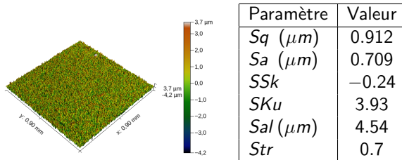
Figure: Surface obtained by honing ( z \times 5 ), WLI, L = 0.9\text{mm} , \Delta x = 0.9\mu\text{m} .
