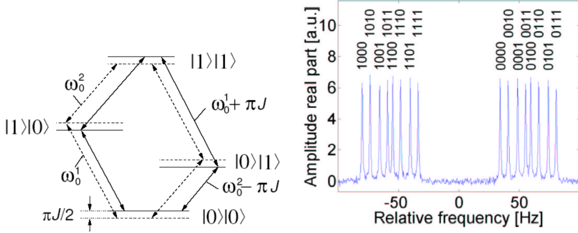
Fig. IV.7. Level scheme of uncoupled and coupled qubits system and NRM spectrum of coupled qubits.
