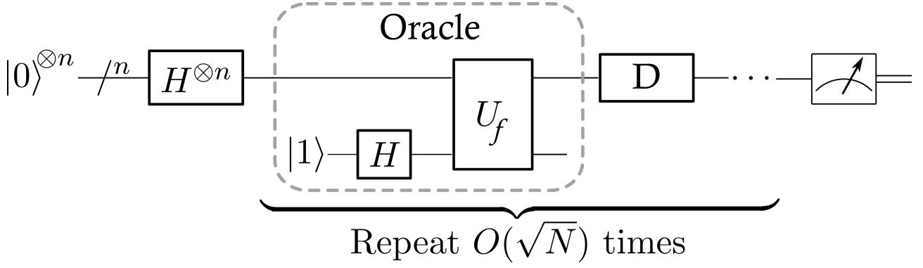
Fig. V.2. Circuit diagram of Grover's algorithm.
