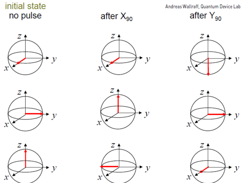
Fig. IV.17. Principle of quantum state tomography.
