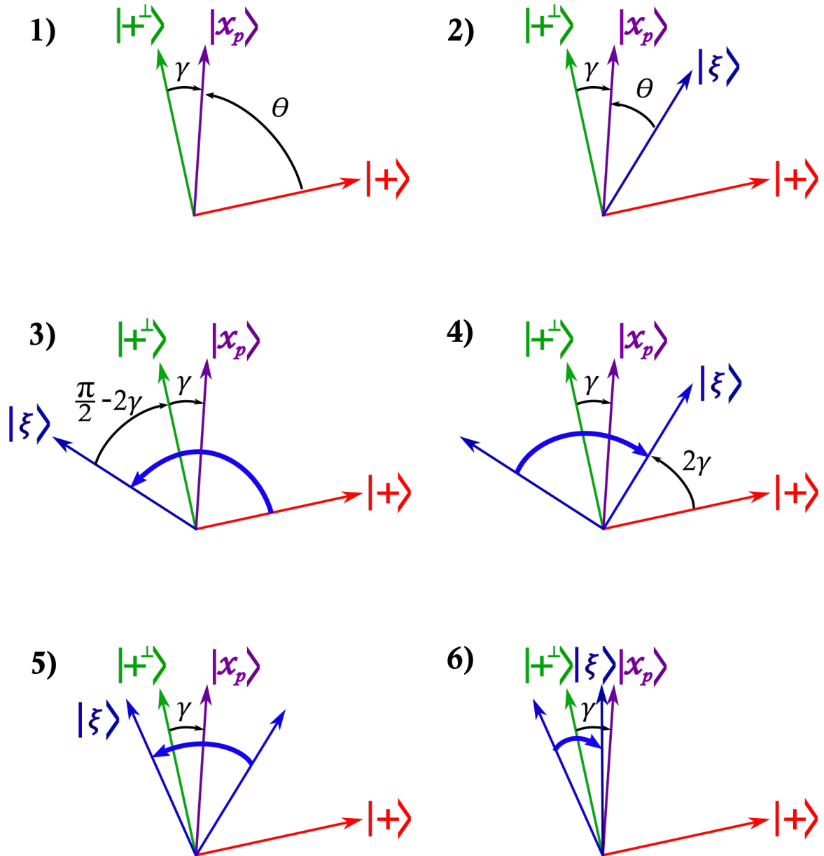
Fig. V.3. Geometrical interpretation of Grover's algorithm.
