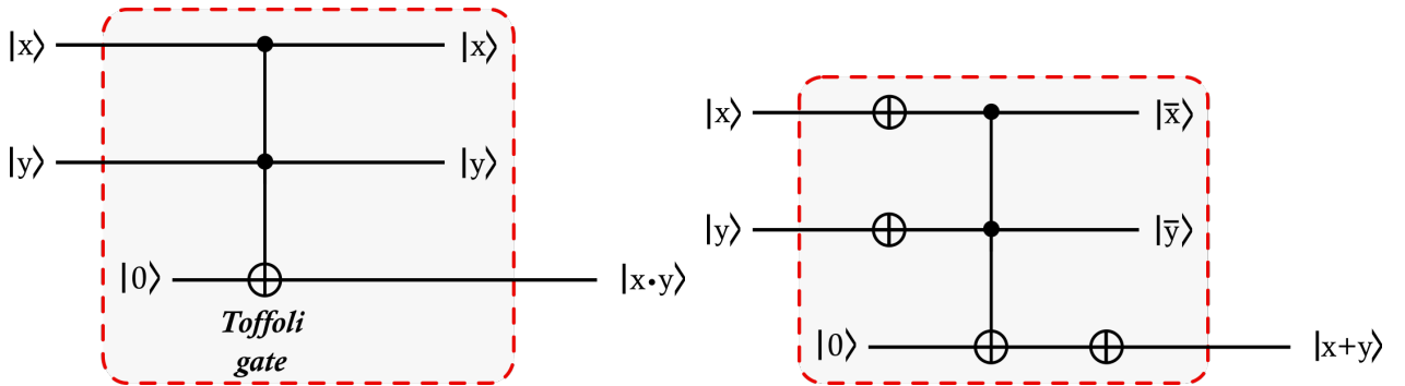
Fig. III.9. AND and OR logical gates based on quantum circuits.
