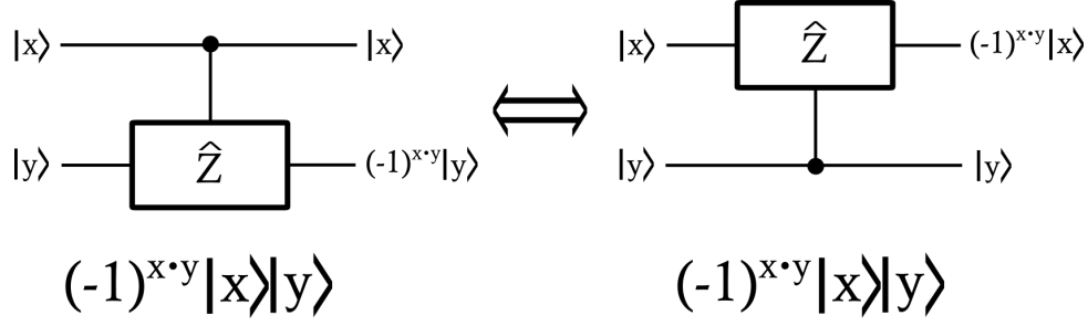
Fig. III.6. C-Z gate.
