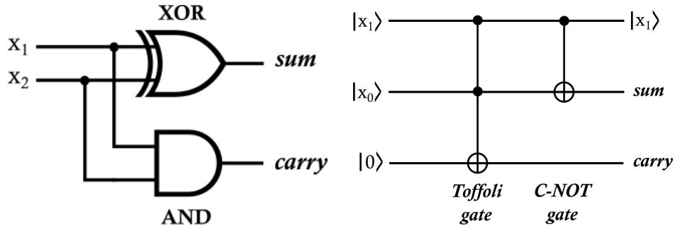
Fig. III.4. Classical and quantum half-adder.
