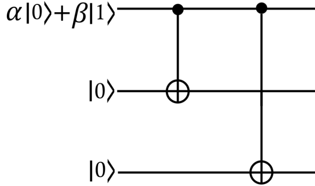
Fig. V.8. Implementation of operator \hat{E} .
