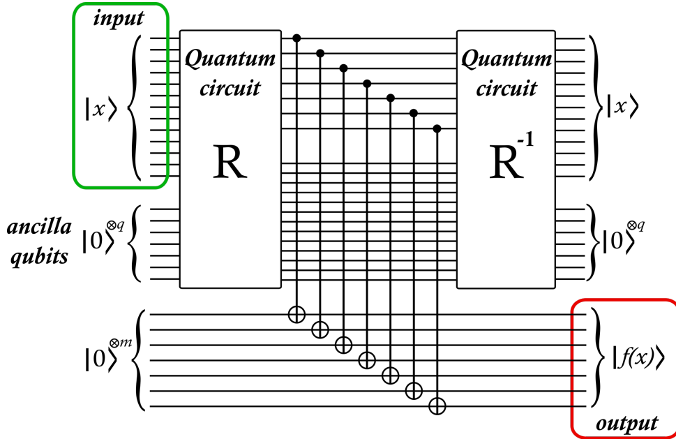
Fig. III.12. Quantum circuit emulating a boolean circuit that performs the function f : \mathbb{F}_n \rightarrow \mathbb{F}_m with ancilla qubits recycling.
