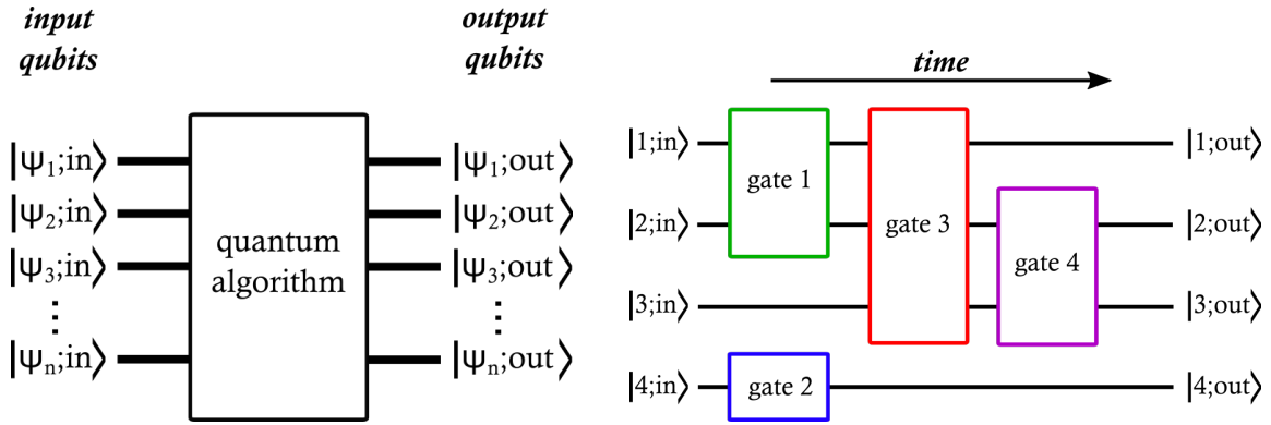
Fig. II.2. Quantum algorithm - I/O approach. Example of quantum circuit.
