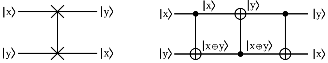
Fig. III.8. SWAP gate and its implementation with 3 C-NOT gates.
