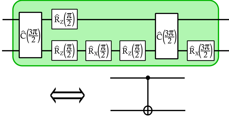
Fig. IV.2. Circuit representation of a C-NOT gate made with a two-qubit interaction \hat{C}(\gamma) .
