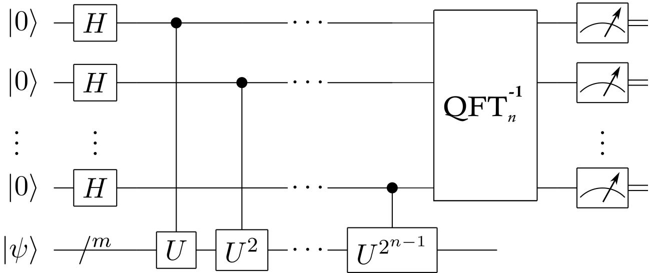
Fig. V.4. Circuit diagram of Quantum Phase Estimation algorithm.
