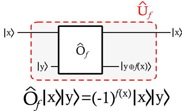
Fig. III.13. Implementation of an oracle. |y\rangle is an ancilla qubit.
