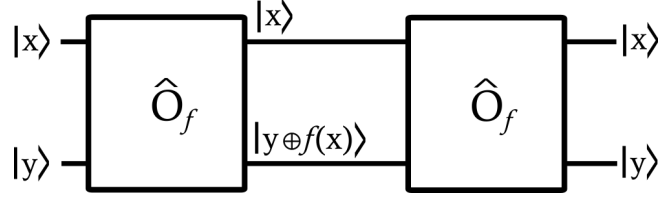
Fig. III.15. Oracle for Deutsch and Deutsch-Josa algorithm is reversible.
