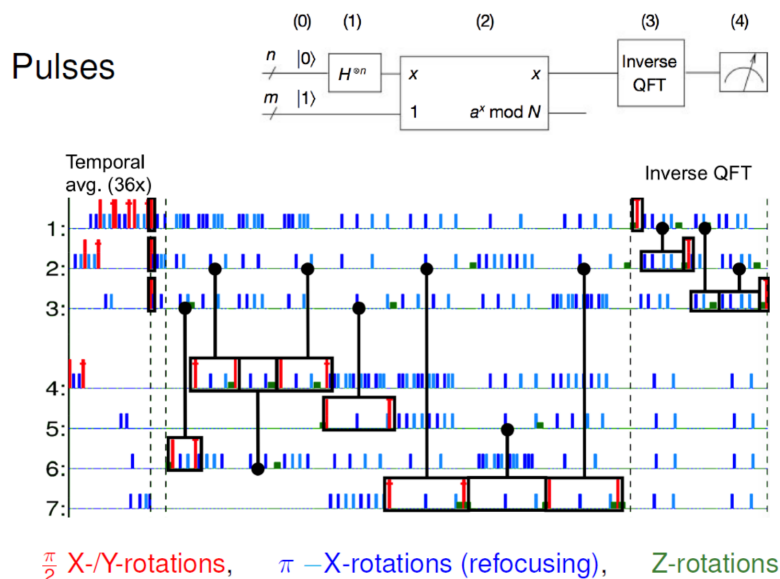
Fig. IV.15. Shor's algorithm: experimental sequence. Extracted from [27].
