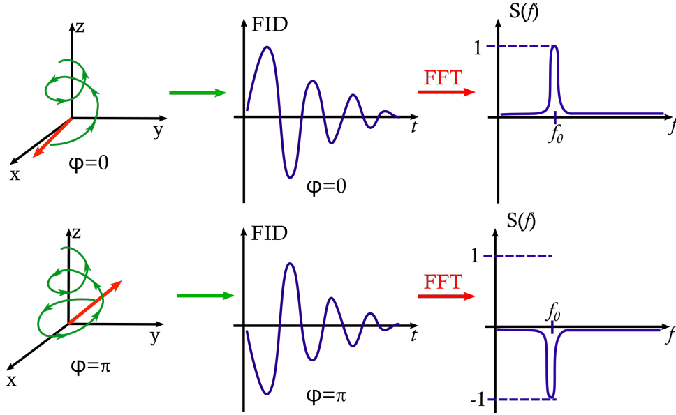
Fig. IV.11. Read-out of the qubit state in the case of NMR implementation : influence of the initial state on the FID signal and its FFT.
