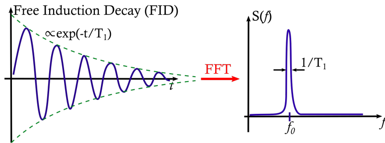
Fig. IV.10. Read-out of the qubit state in the case of NMR implementation : free induction decay (FID) and its FFT to recover spectrum.
