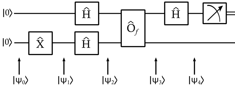
Fig. III.16. Implementation of Deutsch algorithm.
