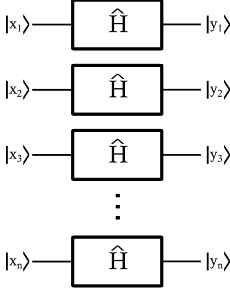
Fig. II.4. Hadamard gate on a quantum register to generate states superposition.
