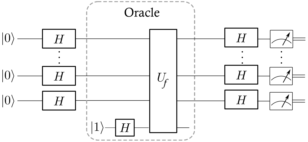
Fig. V.1. Circuit diagram of Bernstein-Vazirani algorithm.
