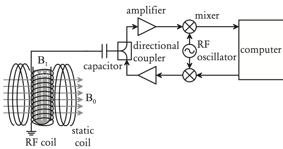
Fig. IV.4. Experimental setup for NMR qubits implementation.
