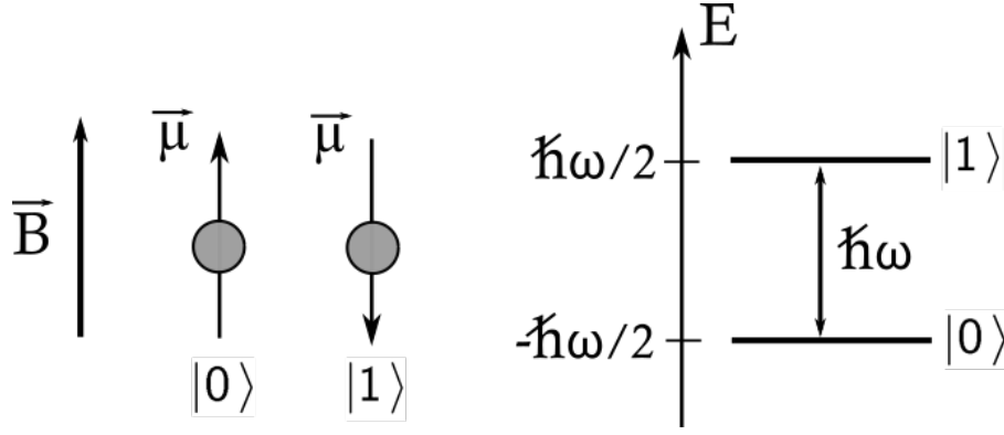
Fig. I.2. Electronic spin in a B field as a two-level system.
