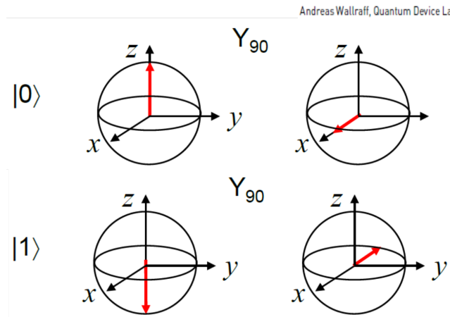
Fig. IV.12. Read-out of the qubit state in the case of NMR implementation.
