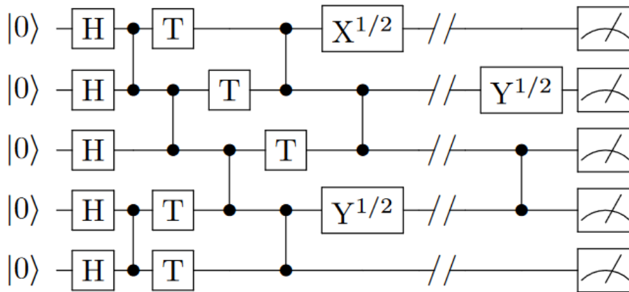
Fig. VI.2. Example of a random quantum circuit in a 1D array of qubits. Vertical lines correspond to controlled-phase (C-Z) gates. Extracted from [6].
