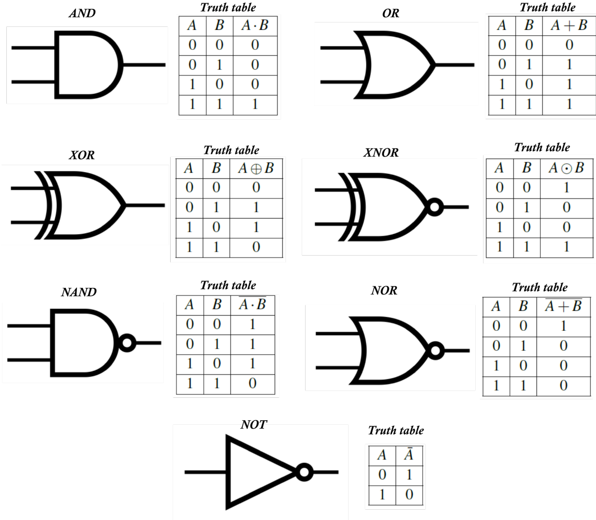
Fig. I.1. Symbolic representation of classical logical gates and corresponding truth tables: AND, OR, XOR, XNOR, NAND, NOR and NOT gates.
