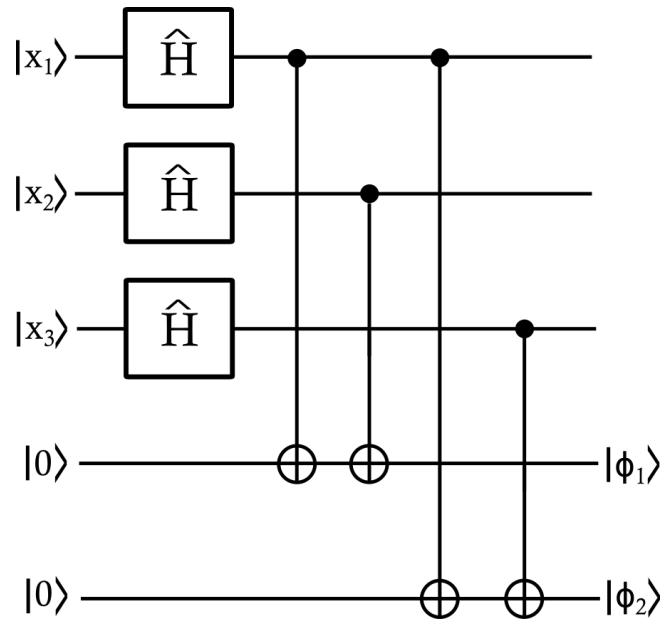
Fig. V.11. Decoding circuit of error correcting code of Fig. V.10.
