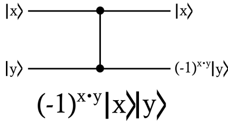
Fig. III.7. C-Z gate compact representation.
