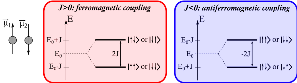
Fig. IV.1. Two spins in interaction: ferromagnetic and anti-ferromagnetic coupling.
