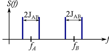
Fig. IV.13. Spectrum of two coupled qubits in their four computational basis states.
