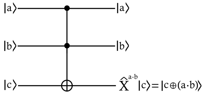
Fig. III.3. Toffoli gate.
