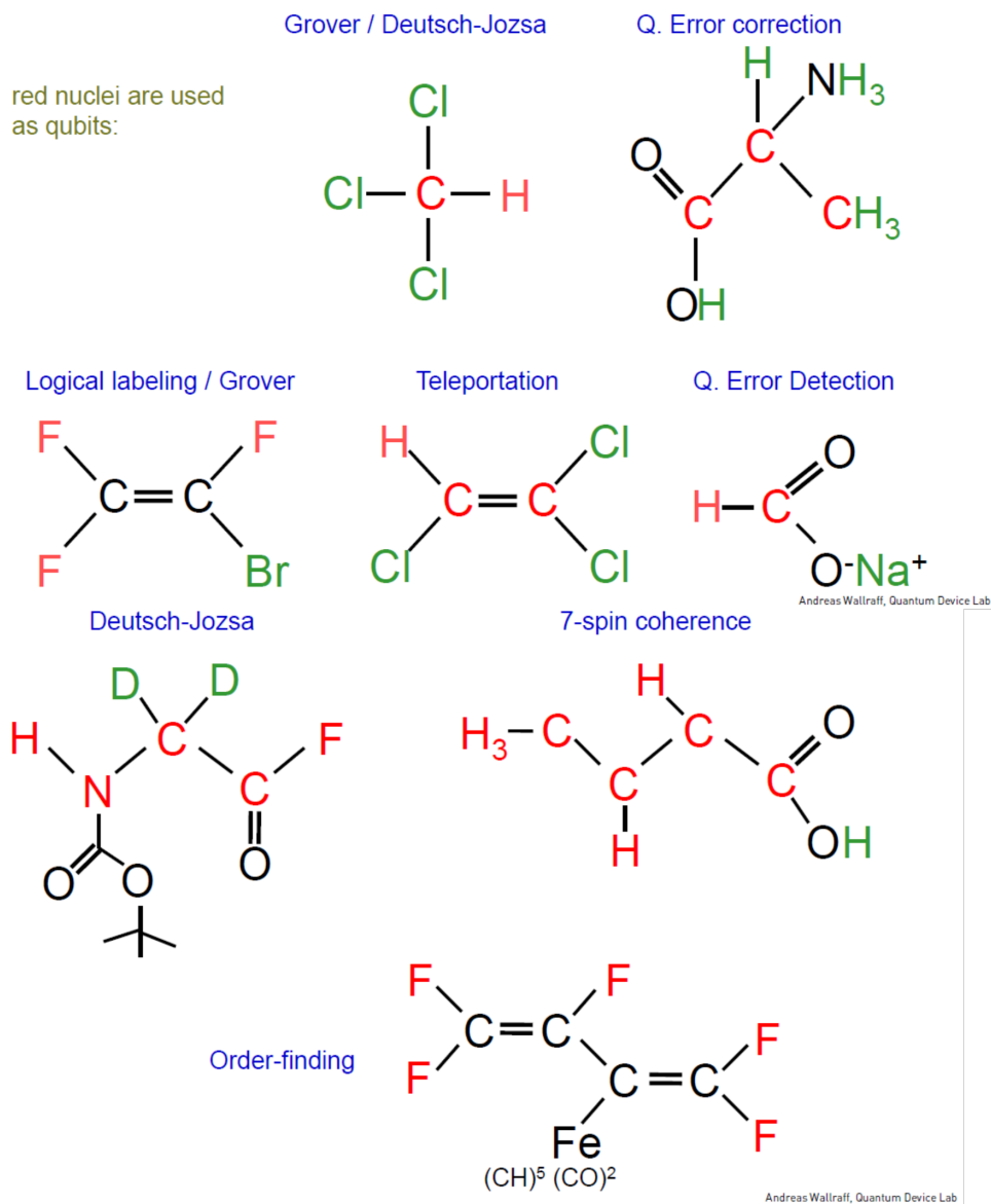
Fig. IV.18. Several molecules used for quantum algorithm implementation by NMR technics (from Andreas Walralf Quantum Device Lab, ETH Zürich, Switzerland).
