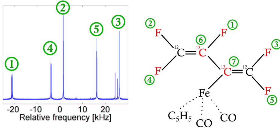
Fig. IV.5. Chemical shifts of the five F qubits of perfluorobutandienyl iron complex.
