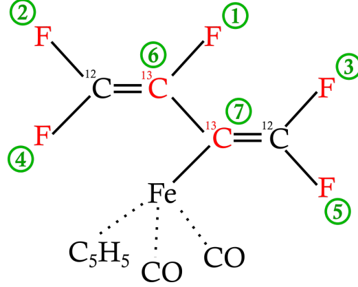
Fig. IV.3. Case of C_4F_5Fe(CH)_5(CO)_2 - perfluorobutadienyl iron complex [27]. Nuclei labeled in red are qubits (F and ^{13}C ), numbered in green. B_0 = 11.7T .
