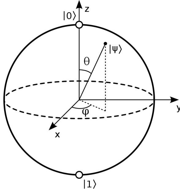
Fig. II.1. Bloch's sphere representation of a qubit.
