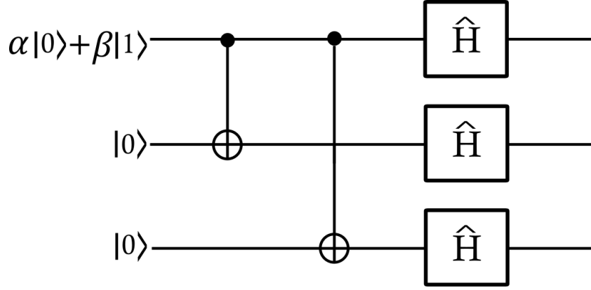
Fig. V.10. More elaborated error correcting code.
