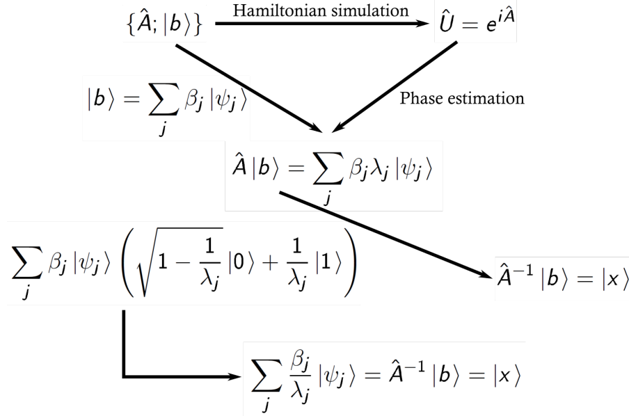
Fig. V.5. HHL algorithm outline.
