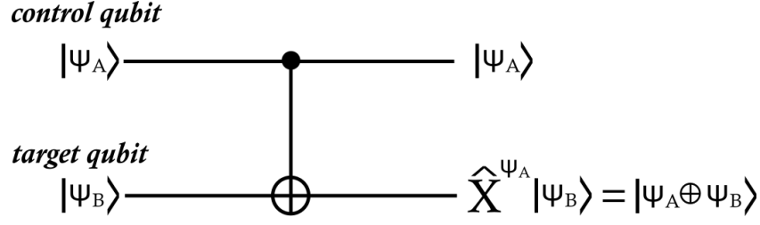
Fig. III.2. C-NOT gate.
