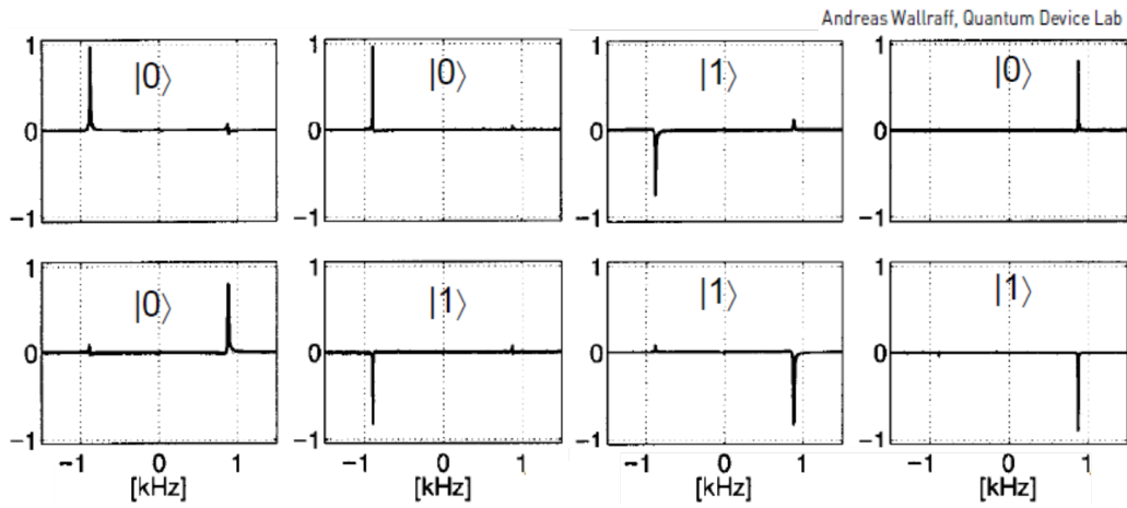
Fig. IV.14. Experimental signal of state read out in NRM implementation (figure from Andreas Waltraff Quantum Device Lab).
