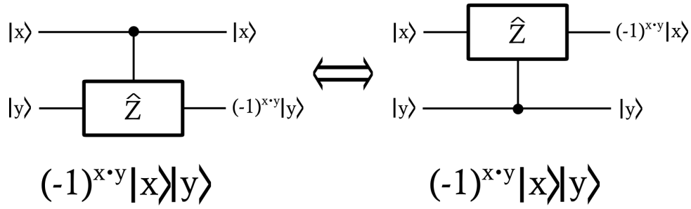
Fig. III.6. C-Z gate.
