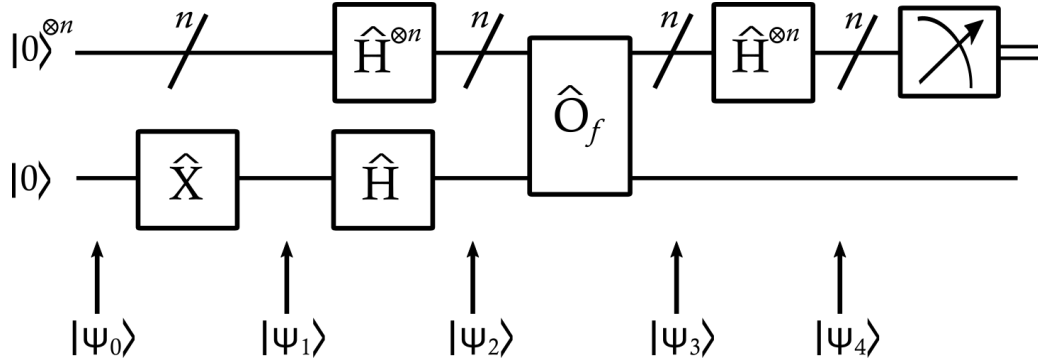
Fig. III.17. Implementation Deutsch-Jozsa algorithm.
