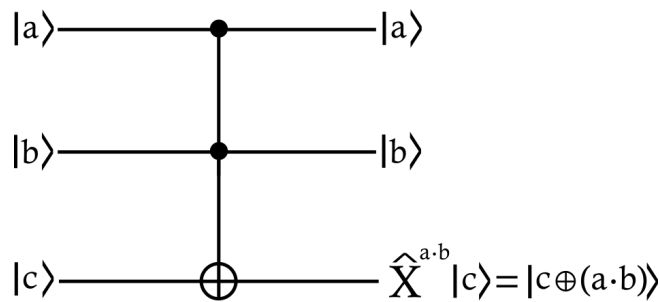
Fig. III.3. Toffoli gate.
