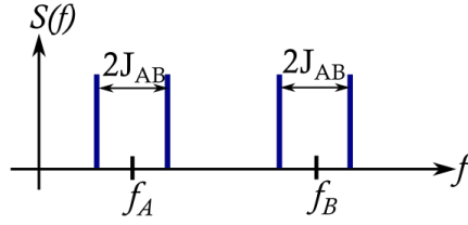
Fig. IV.13. Spectrum of two coupled qubits in their four computational basis states.
