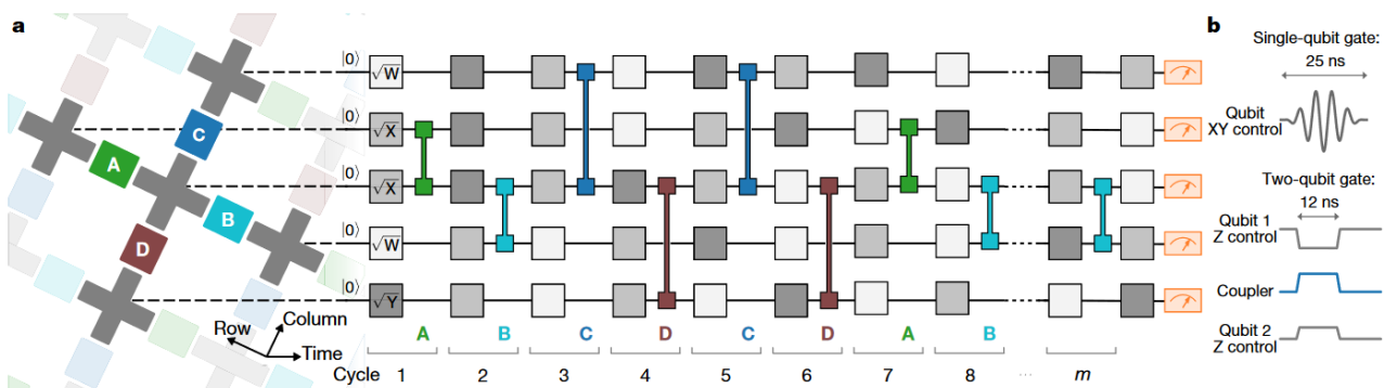
Fig. 3 | Control operations for the quantum supremacy circuits. a , Example quantum circuit instance used in our experiment. Every cycle includes a layer each of single- and two-qubit gates. The single-qubit gates are chosen randomly from \{\sqrt{X}, \sqrt{Y}, \sqrt{W}\} , where W = (X + Y)/\sqrt{2} and gates do not repeat sequentially. The sequence of two-qubit gates is chosen according to a tiling pattern, coupling each qubit sequentially to its four nearest-neighbour qubits. The
