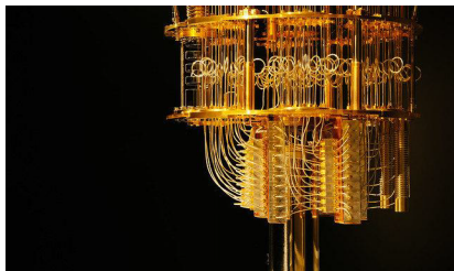
Photo of a IBM quantum computer with 53 qubits chip. (Picture credits: IBM research).
