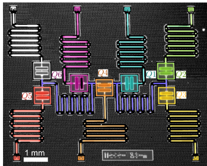
Photography of the chip used in IBM's quantum computer used for \text{BeH}_2 quantum chemistry simulation.
