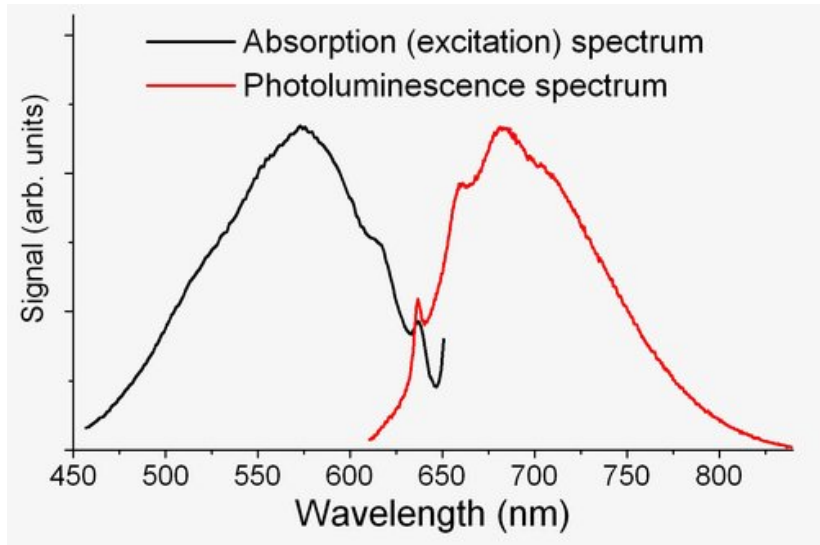
Absorption and emission spectrum of NV center
