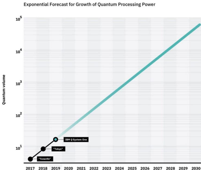
IBM Quantum Volume Growth Chart
