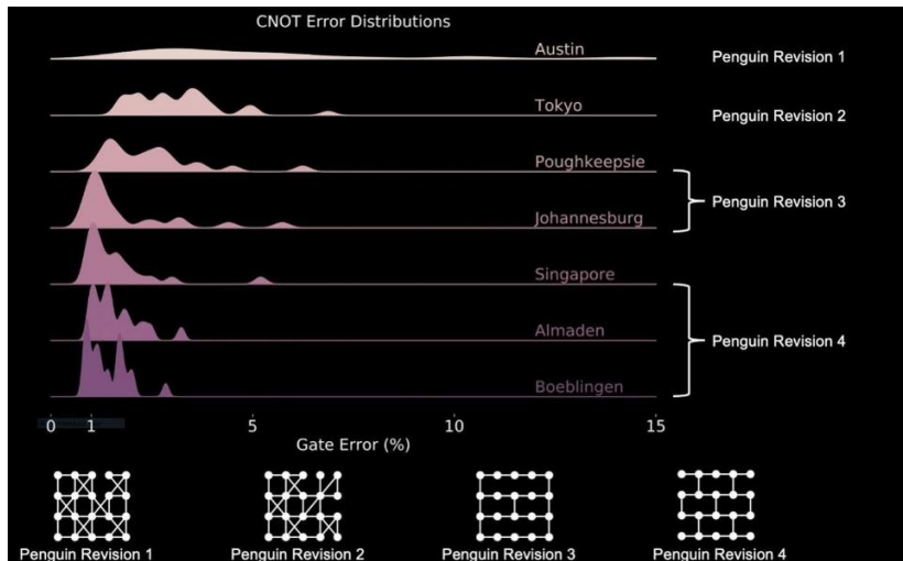
CNOT Error Distributions for different version of IBM's 20-qubits systems.
